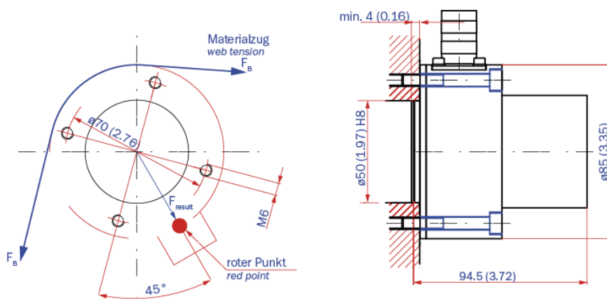
Figure 4: dimension machine frame for PH mount
