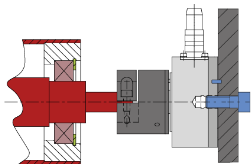
Figure 5: Flat mount
