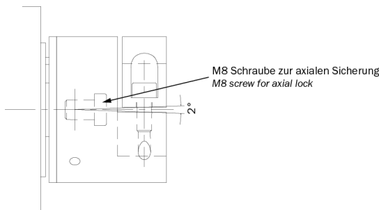
Figure 8: angular misalignment
